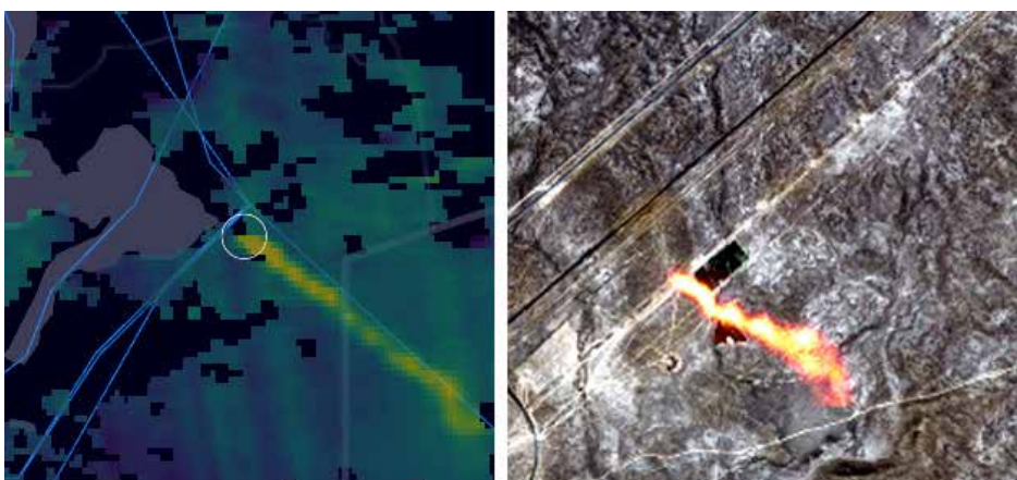
Substantial methodological development is still needed to improve satellite-derived emission estimates, for which accurate measurements on the ground are indispensable. However, with the current capabilities, an important new contribution to regional emission monitoring can already be made. The combination of Sentinel-5P and Sentinel2 Methane measurements show promising results in deriving emission rates (see Figure 5).
