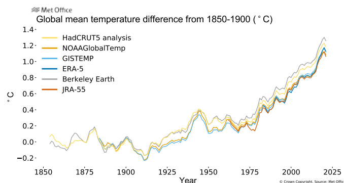
Figure 1. Five-year running average of global temperature anomalies (relative to pre-industrial) from 1854 to 2021 for six data sets: HadCRUT.5.0.1.0, NOAA GlobalTemp v5, GISTEMP v4, Berkeley Earth, ERA5, and JRA-55. Data for 2020 to June 2021 for HadCRUT5 and July for NOAA GlobalTemp, GISTEMP, Berkeley Earth, ERA5 and JRA-55.
